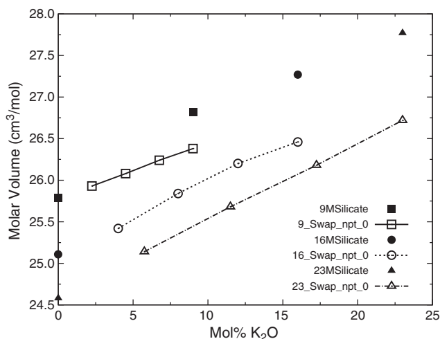
Fig. 3. Molar volumes of as-formed and ion-exchange simulated glasses. Data points at 0 mol% \text{K}_2\text{O} are for as-formed sodium silicate systems ( x NaSilicate), where x=23 and x=9 have the lowest and highest molar volumes, respectively. Molar volume error bars are within the symbol height.
