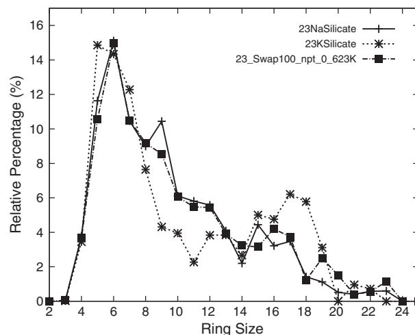
Fig. 2. Ring size distributions for x=23 mol% end-member and ion-exchange simulated glasses. Ion-exchange stuffing is carried out at 623 K and the structure is analyzed at 300 K. Note, traces for 23NaSilicate and 23_Swap100_npt_0_623K largely overlap for all ring sizes.
